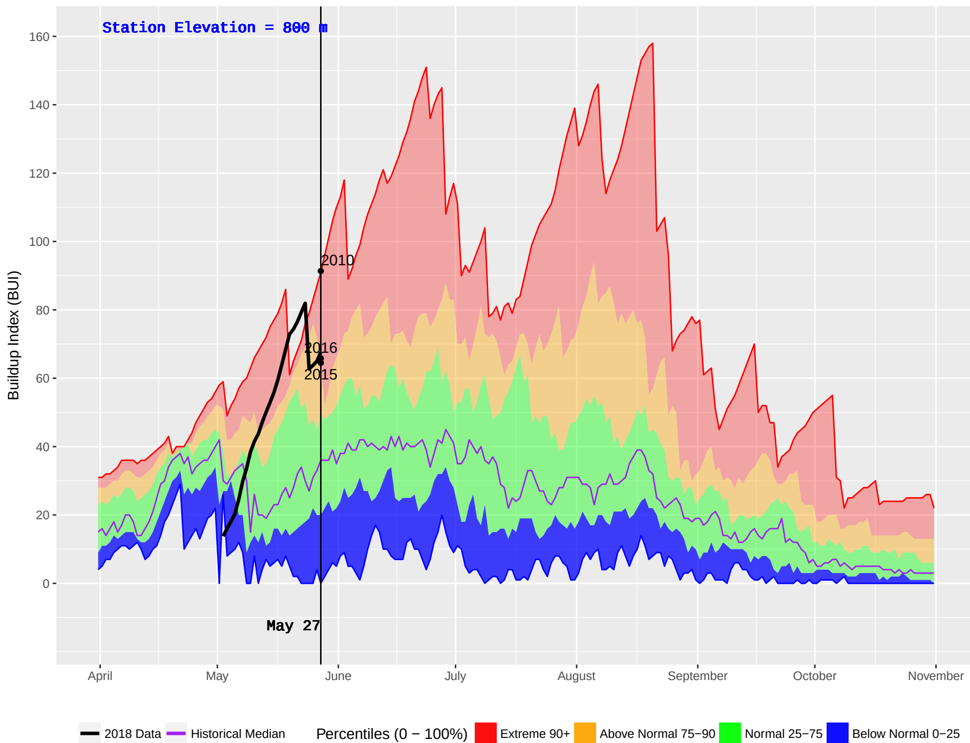
DEASE LAKE FS (108) : Historical (1978–2016) and Current (2018) Noon Buildup Index (BUI)
