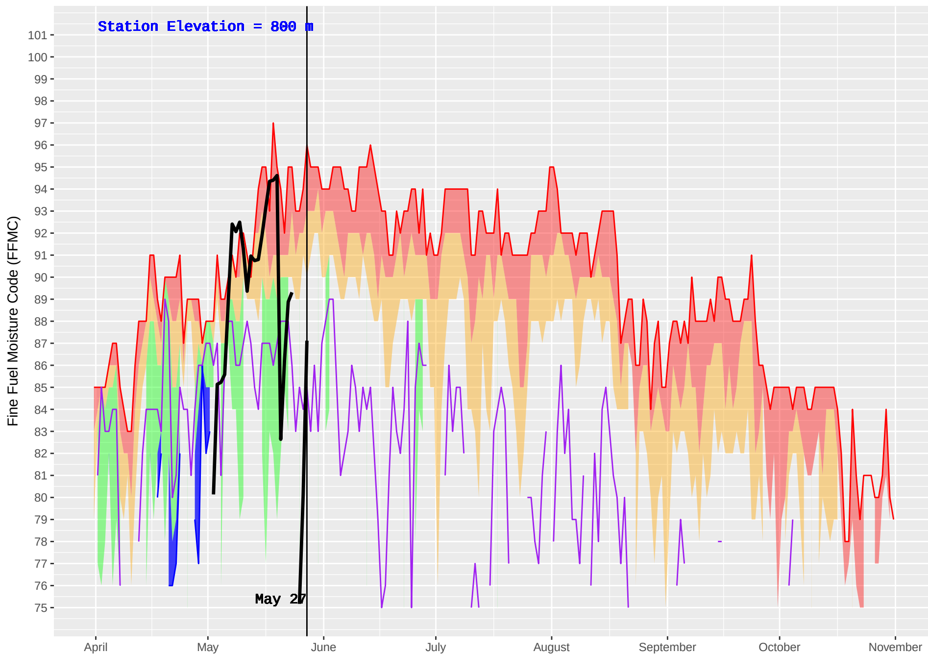
DEASE LAKE FS (108) : Historical (1978–2016) and Current (2018) Noon Fine Fuel Moisture Code (FFMC)
