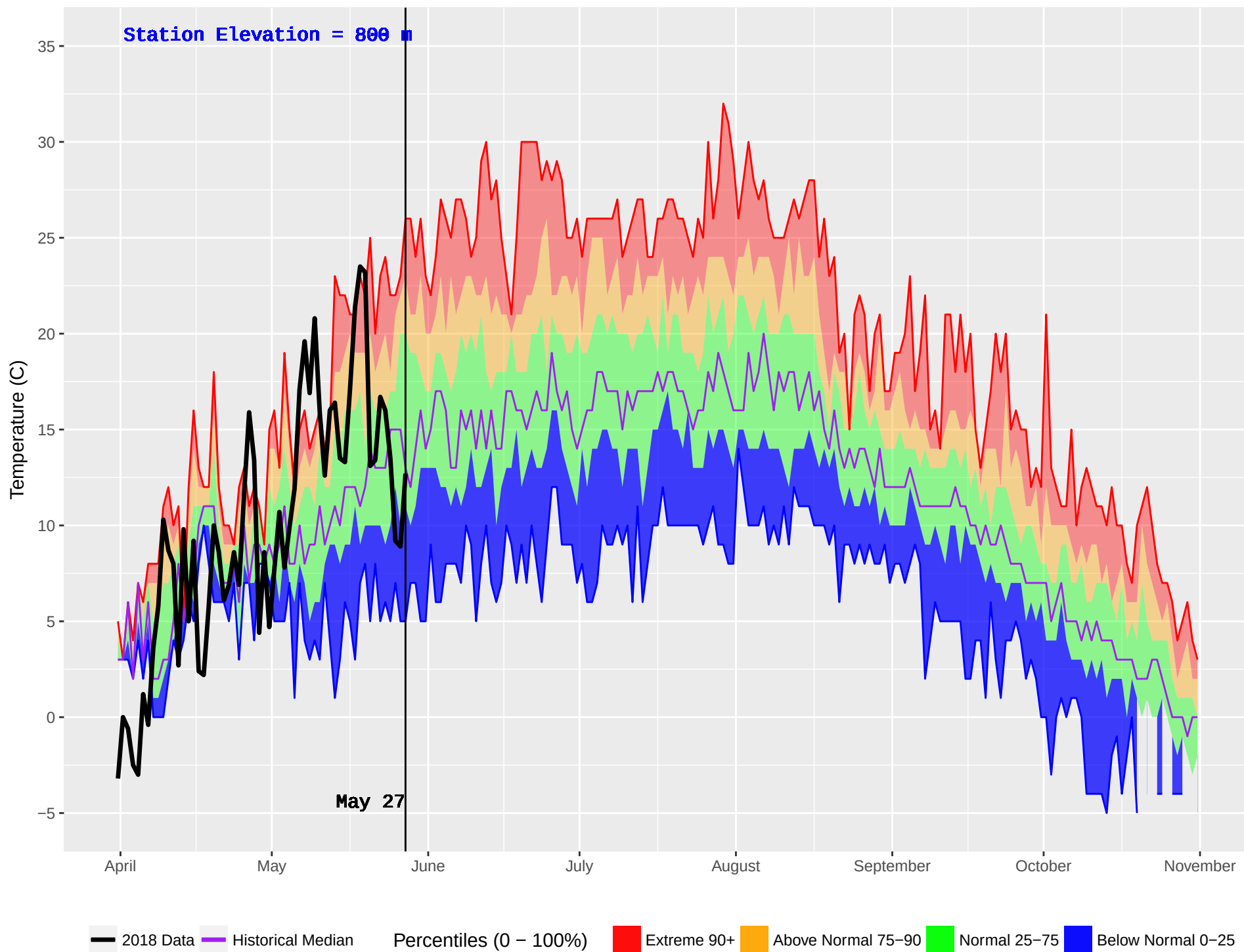
DEASE LAKE FS (108) : Historical (1978–2016) and Current (2018) Noon Temperature
