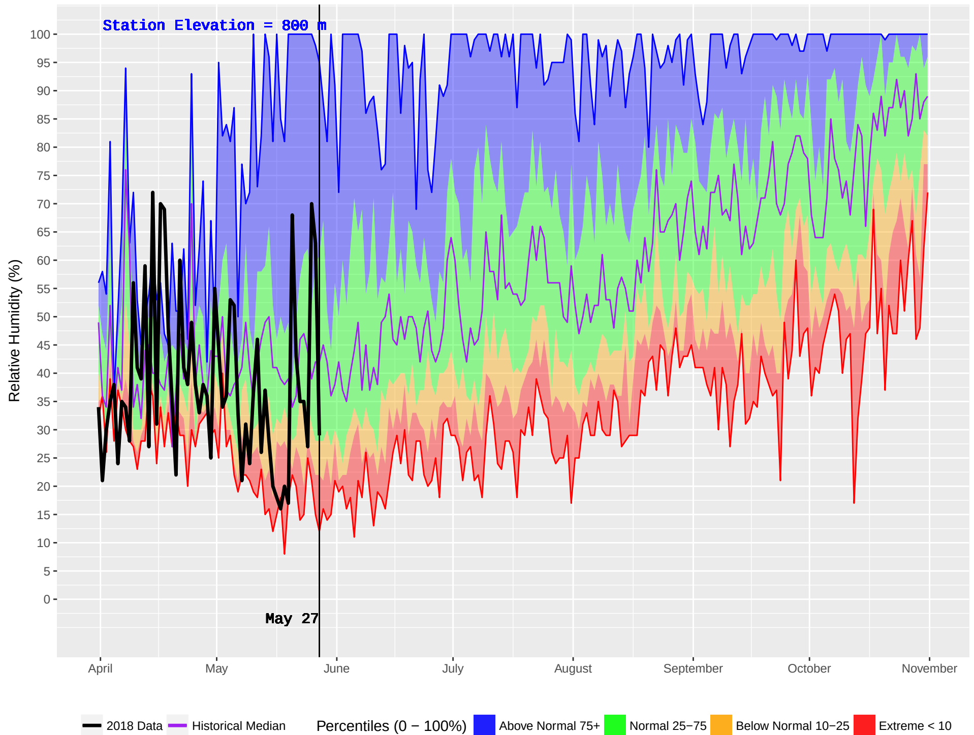
DEASE LAKE FS (108) : Historical (1978–2016) and Current (2018) Noon Relative Humidity
